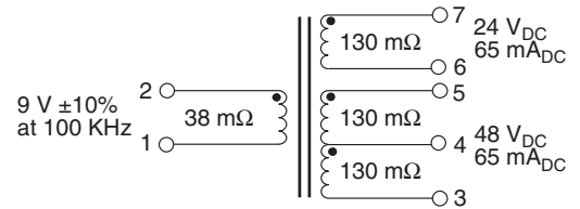
FLYBACK TRANSFORMER (approximately 10° C temperature rise)
