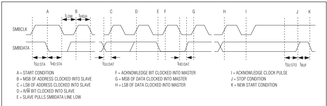
Figure 4. Read-Timing Diagram
