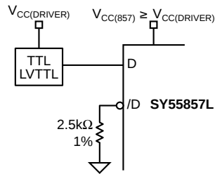
Figure 3. 3.3V "TTL"
