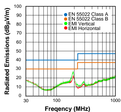
Radiated Emissions EN55022 compliant: V_{IN} = 24V ; V_{OUT} = 5V Load = 2A
