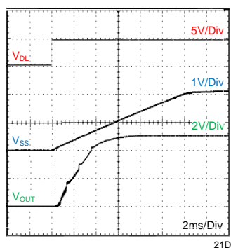
Deadlock start-up I_{OUT} = 2A
