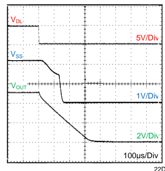
Deadlock shut-down I_{OUT} = 2A
