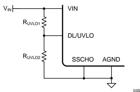
Figure 2. Under voltage Lockout (UVLO) Schematic
