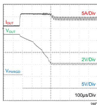
Figure 15. Overcurrent Limiting
