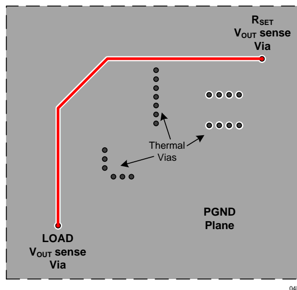
Figure 5. Layout bottom layer
