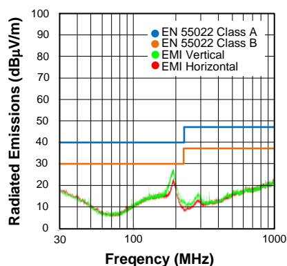
Figure 15. Radiated Emissions EN55022 complaint: V_{IN} = 24V ; V_{OUT} = 5V ; Load 2A
