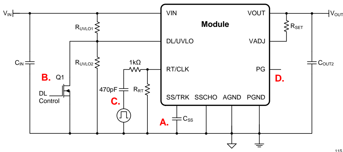
Figure 6. Schematic for optional functions
