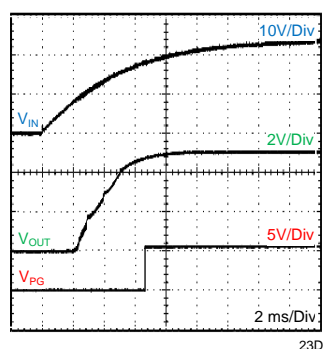
Startup V_{IN} = 10V ; I_{OUT} = 2A
