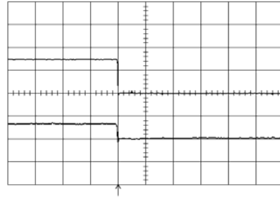
Shut-down enabled by disconnecting V_I at: T_{ref} = +25^\circ\text{C} , I_O = 10\text{ A} resistive load, V_I = 3.3\text{ V} . Top trace: output voltage (1.0 V/div.). Bottom trace: input voltage (2 V/div.). Time scale: 5.0 ms/div..
