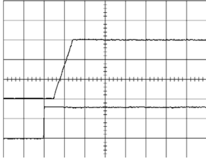
Start-up enabled by connecting V_I at: T_{ref} = +25^\circ\text{C} , I_O = 10\text{ A} resistive load, V_I = 3.3\text{ V} . Top trace: output voltage (0.5 V/div.). Bottom trace: input voltage (2 V/div.). Time scale: 5 ms/div..
