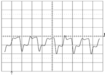
Output voltage ripple (20mV/div.) at: T_{ref} = +25^\circ\text{C} , I_O = 10\text{ A} resistive load, V_I = 3.3\text{ V} . Time scale: 2 \mu\text{s} /div. See the filter in the Output ripple and noise section (EMC Specification).
