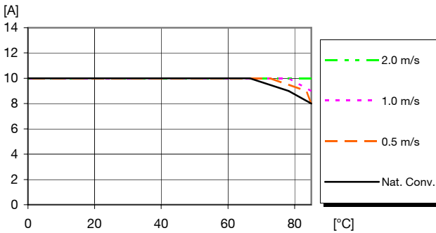
Available load current vs. ambient air temperature and airflow at V_I = 3.3 V, V_{OUT} = 2.5 V . See Thermal Consideration section.
