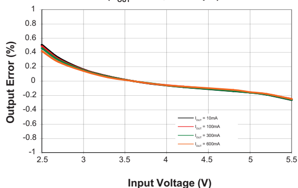
Buck Line Regulation ( V_{OUT} = 1.2V ; L = 2.2\mu H )
