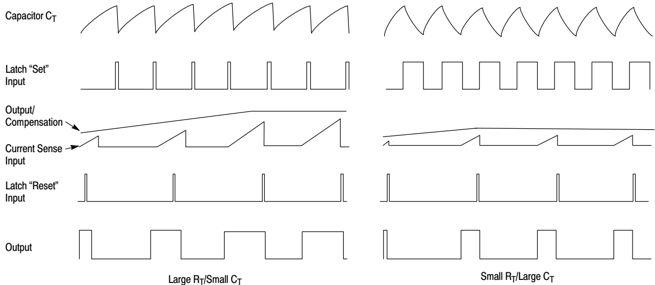
Figure 17. Timing Diagram
