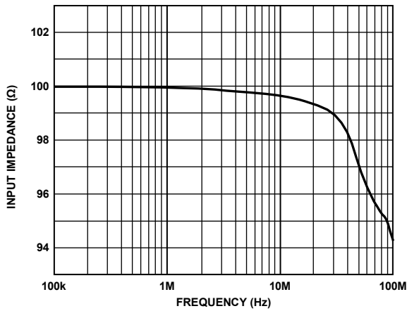
Figure 16. Input Impedance vs. Frequency (Gain = 10 dB)
