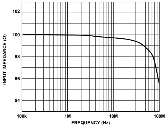
Figure 17. Input Impedance vs. Frequency (Gain = 30 dB)
