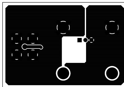
Solder Side
