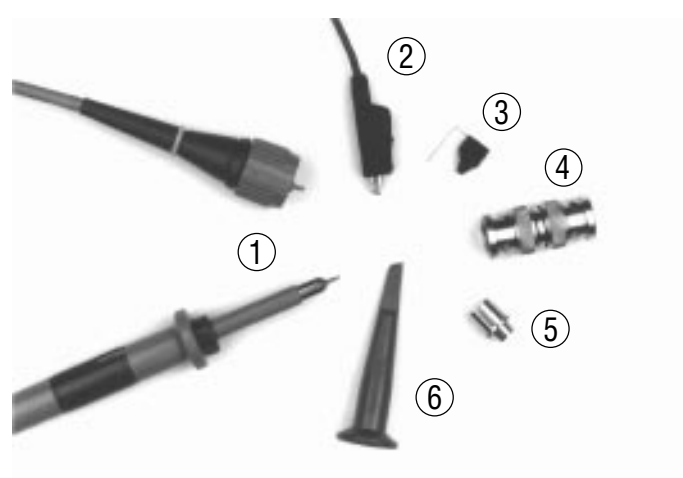
Figure 5: Probe and BNC Accessories
