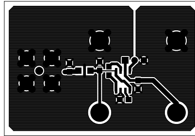
Component Side
