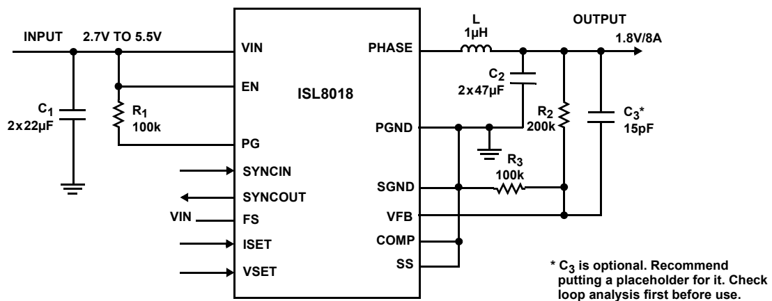
FIGURE 2. TYPICAL APPLICATION DIAGRAM - SINGLE CHIP 8A
