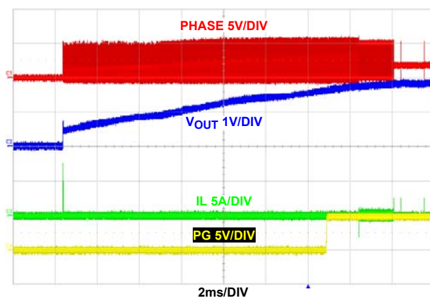
FIGURE 31. OUTPUT SHORT-CIRCUIT RECOVERY
