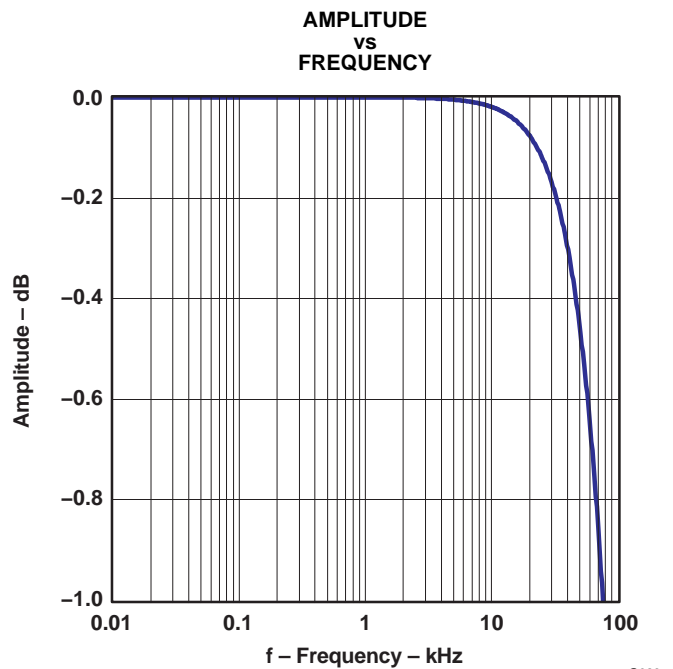
Figure 23. Pass-Band characteristic
