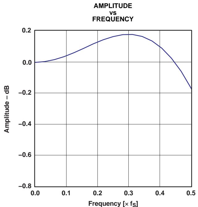
Figure 28. Pass-Band Characteristic
