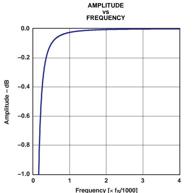
Figure 21. Pass-Band Characteristic
