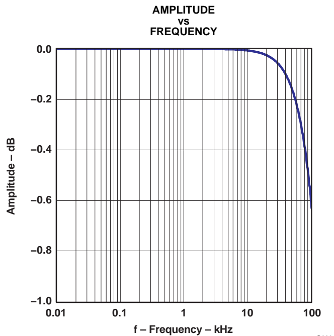
Figure 30. Pass-Band Characteristic
