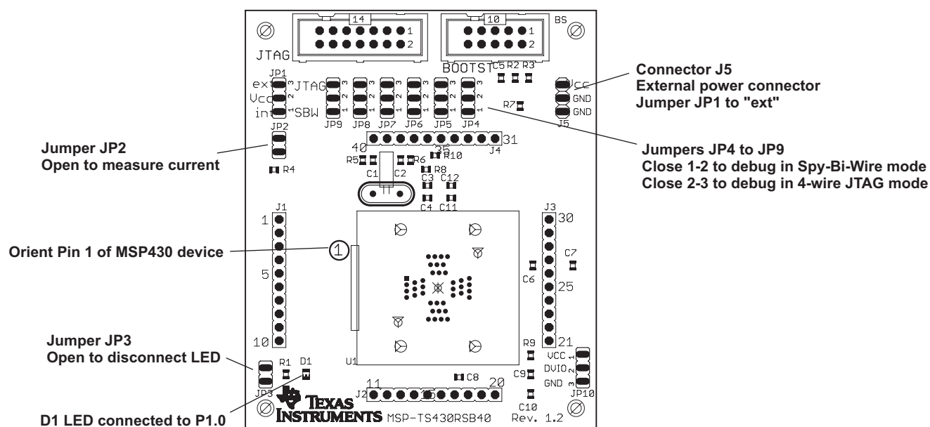
Figure B-20. MSP-TS430RSB40 Target Socket Module, PCB
