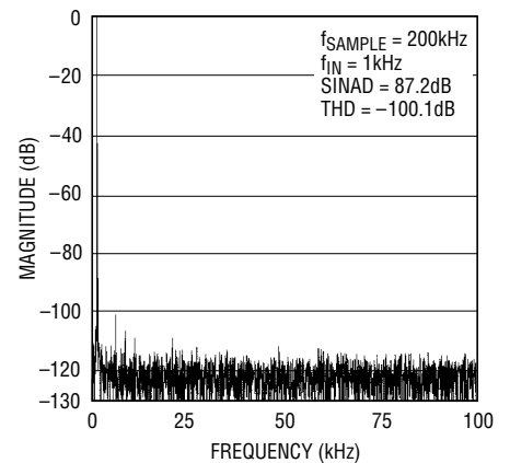
Nonaveraged 4096 Point FFT Plot
