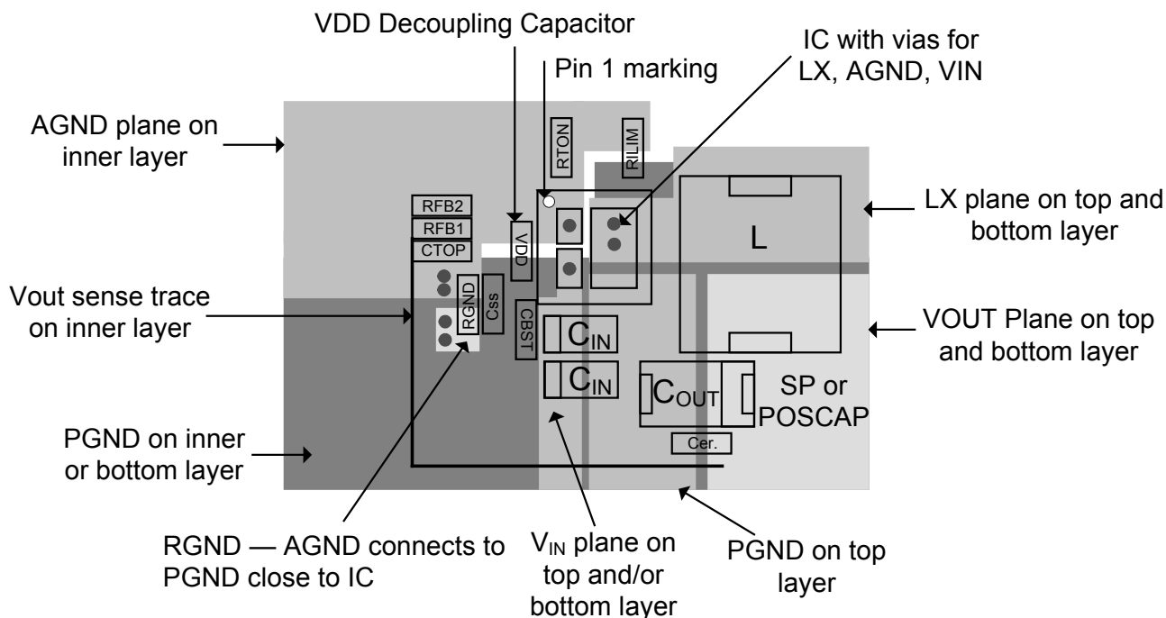
Figure 17 — PCB Layout
