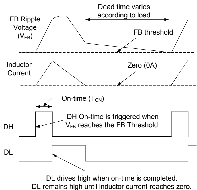
Figure 5 — Power-save Operation
