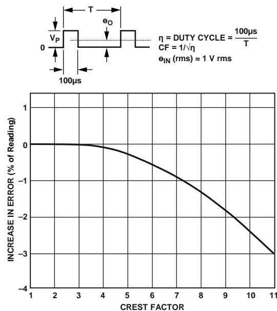
Figure 9. Error vs. Crest Factor
