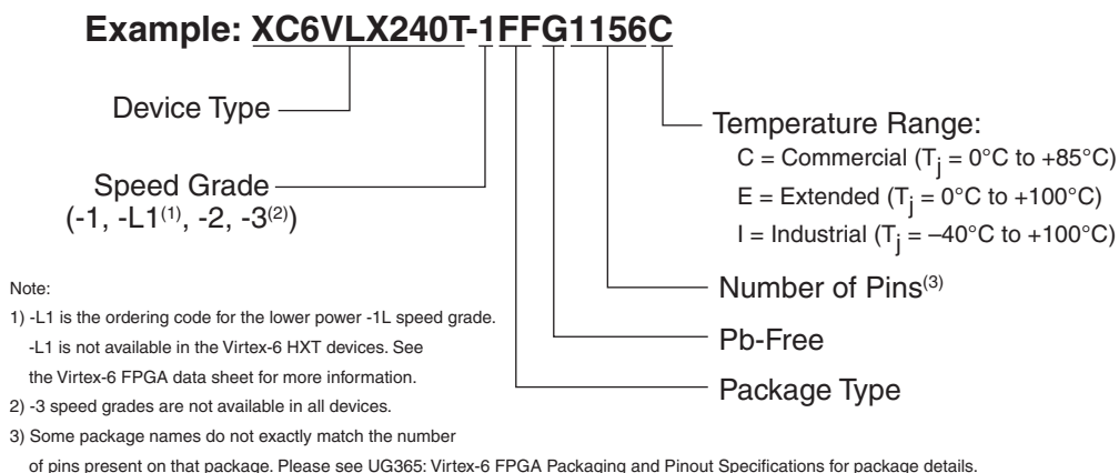
Figure 1: Virtex-6 FPGA Ordering Information
