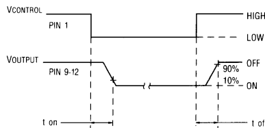
OUTPUT TURN-ON AND TURN-OFF TIMING (A) FIGURE 5
