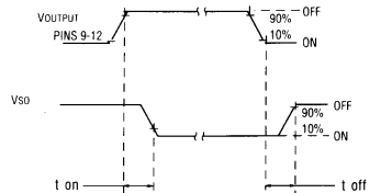
STATUS TURN-ON AND TURN-OFF TIMING (A) FIGURE 6
