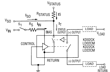
(C) 2 TERMINAL INPUT (DIRECT DRIVE) WITH STATUS
