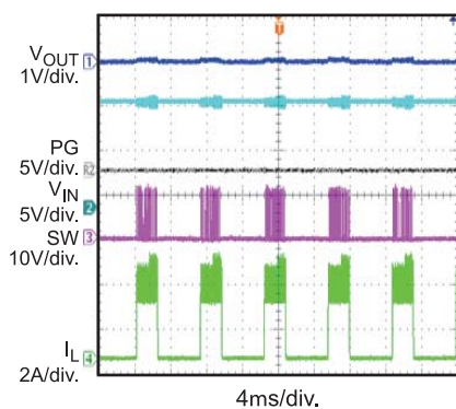
Output Ripple
