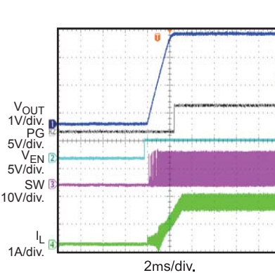
Start-Up through EN/SYNC I_{OUT}=1.5A
