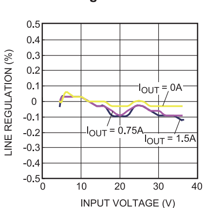
Line Regulation
