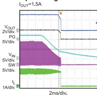
Shutdown through Input Voltage I_{OUT}=1.5A
