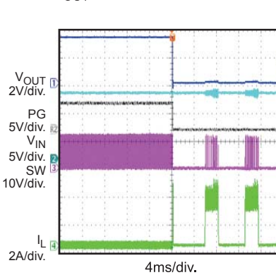
SCP Entry I_{OUT}=0A
