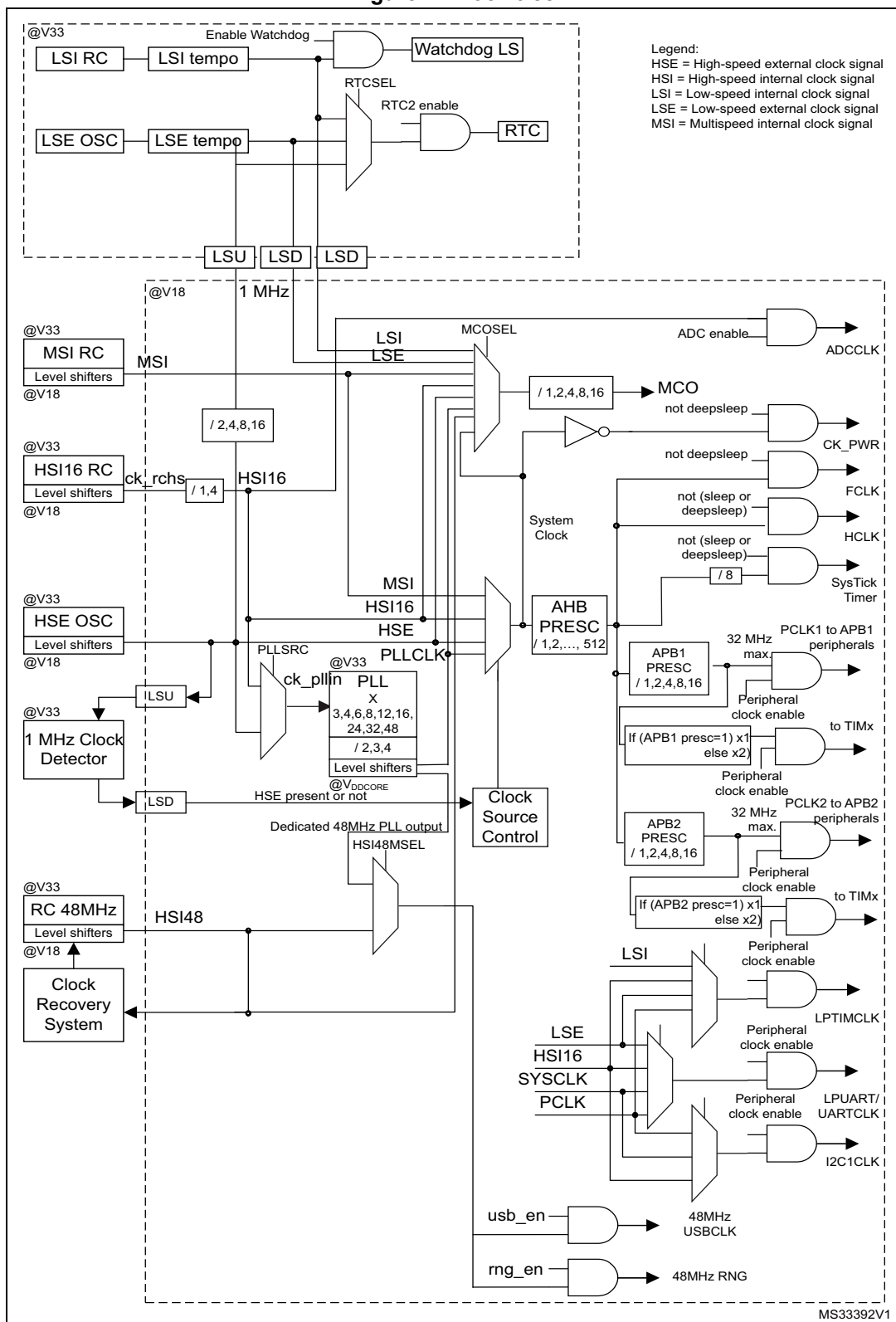
Figure 2. Clock tree
