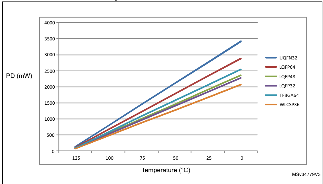
Figure 56. Thermal resistance
