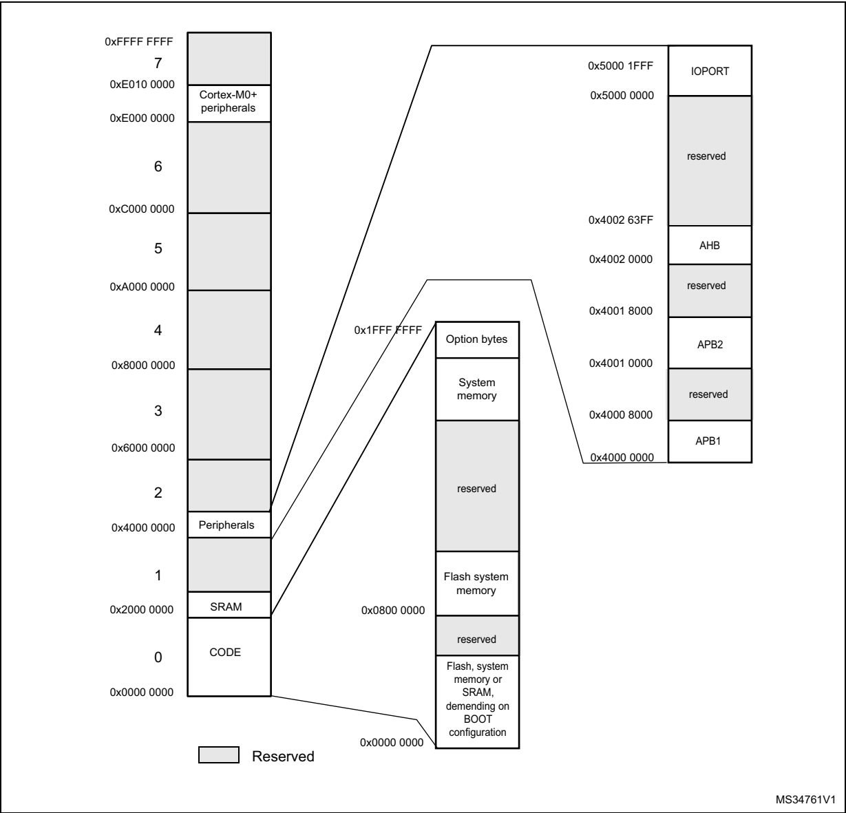
Figure 9. Memory map
