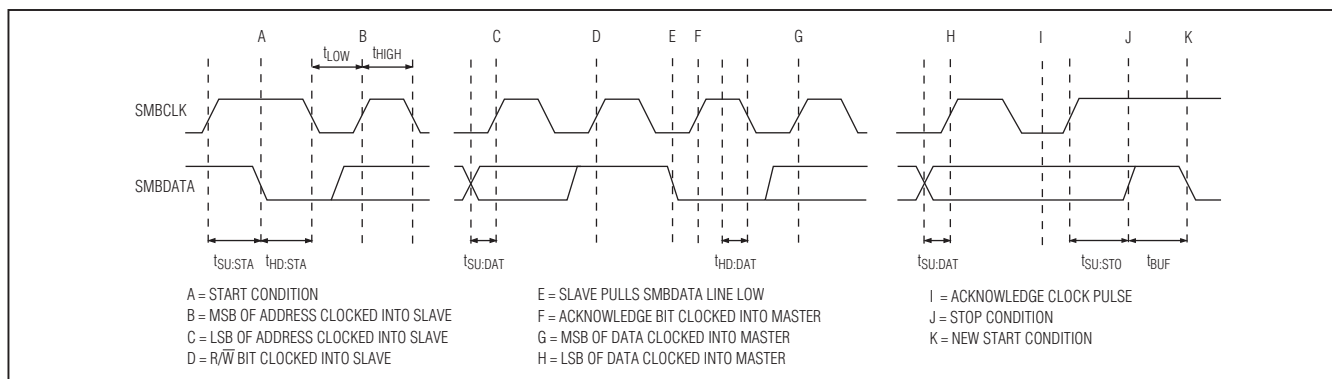
Figure 5. SMBus Read Timing
