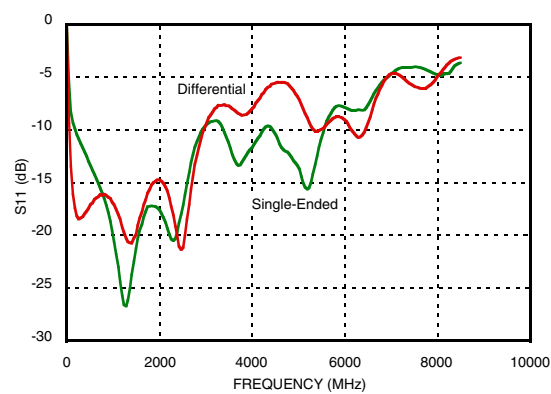
Figure 20. S-Parameters - S11 [11]
