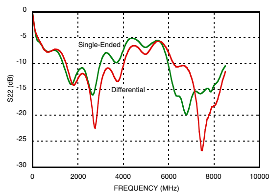
Figure 22. S-Parameters - S22 [11]
