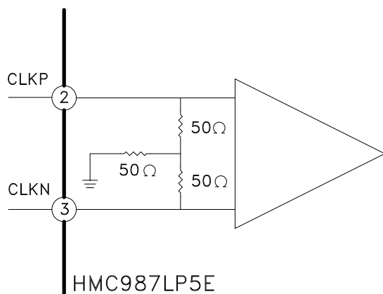
Figure 29. DC Coupled LVPECL Interface
