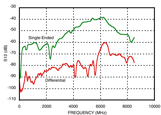
Figure 21. S-Parameters - S12 [11]
