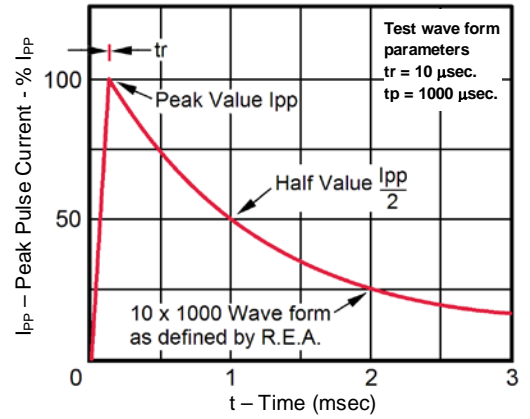
FIGURE 2 – Pulse Waveform
