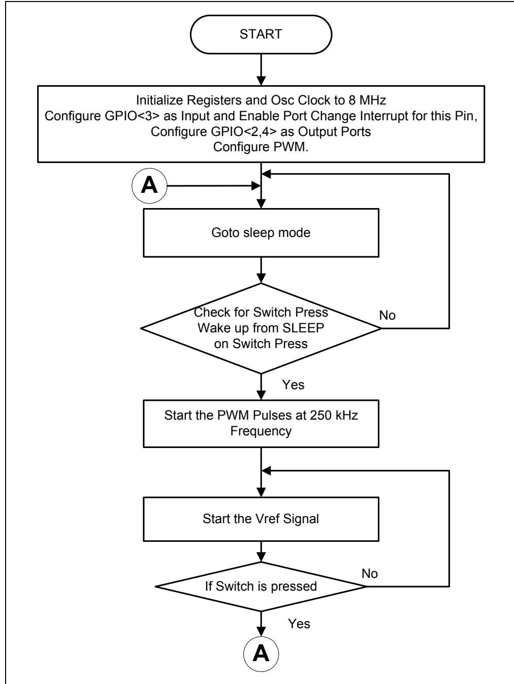
FIGURE C-1: Firmware Flowchart.
