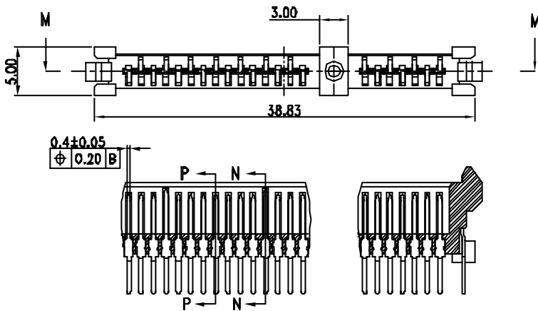
SECTION M-M
