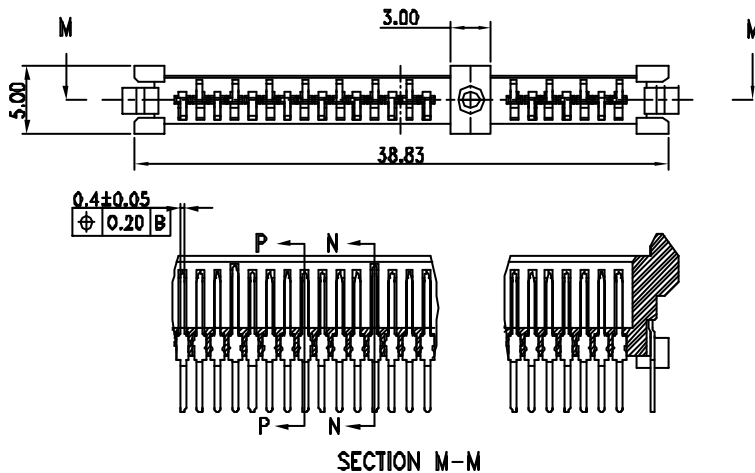
SECTION M-M
