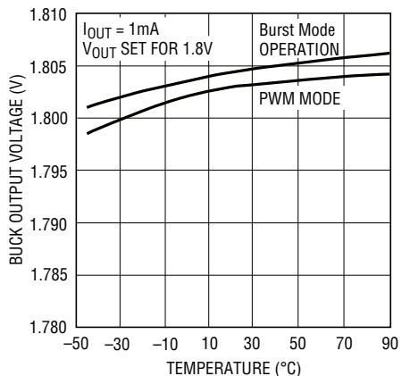
Buck Output Voltage vs Temperature
