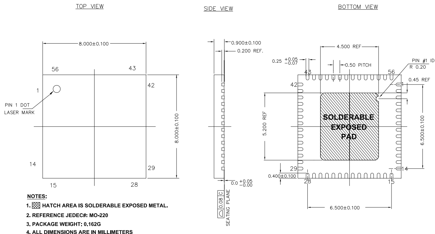
Figure 11-2. 56-Pin QFN 8 × 8 mm Sawn Version (001-53450)
