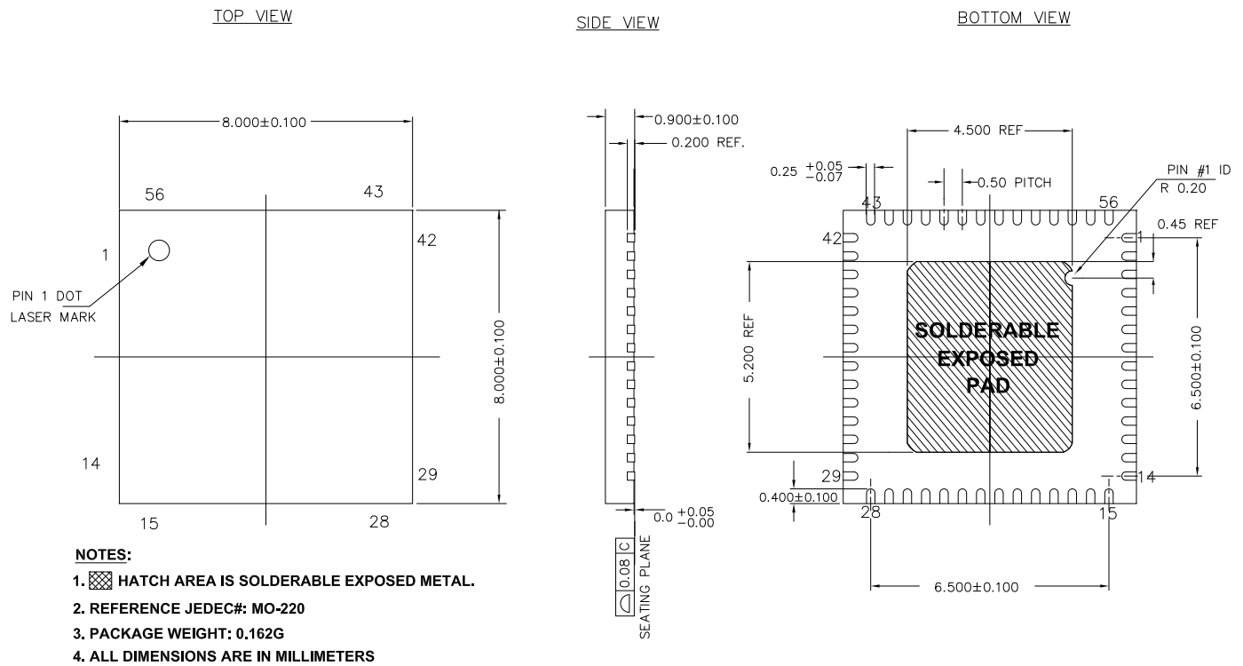
Figure 11-2. 56-Pin QFN 8 × 8 mm Sawn Version (001-53450)
