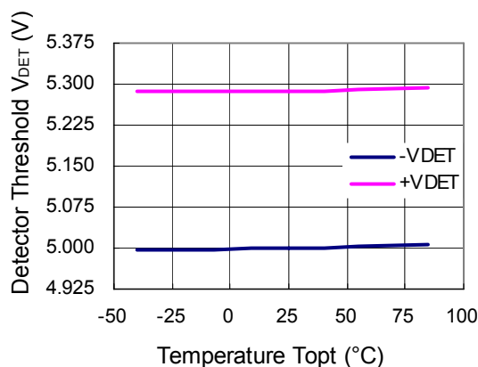
R3118x50xA/C ( V_{\text{DD}}=5.3\text{V} )
