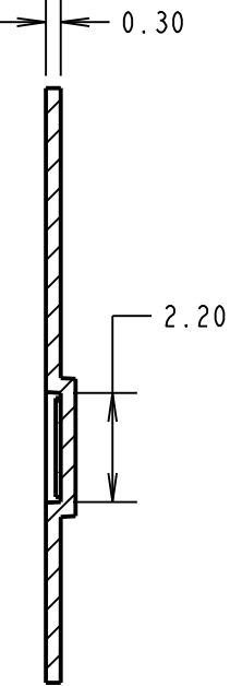
SECTION Y-Y
