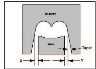
Crimper-to-Anvil Clearance = X + Y at the Final Crimp Height
