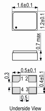
Underside View
