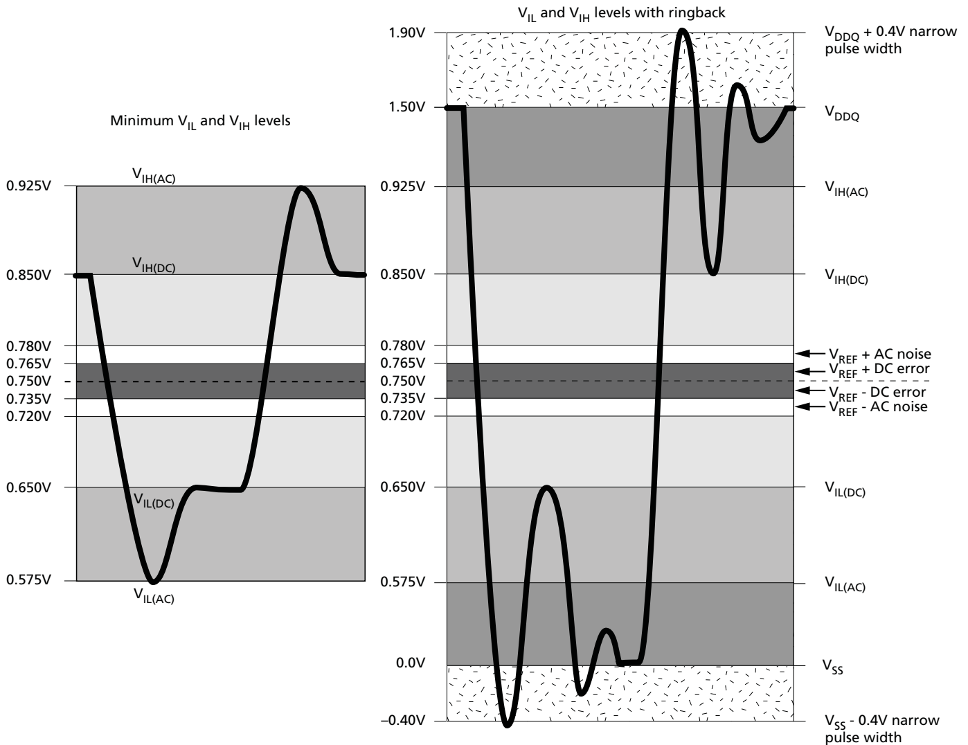
Figure 13: Input Signal
