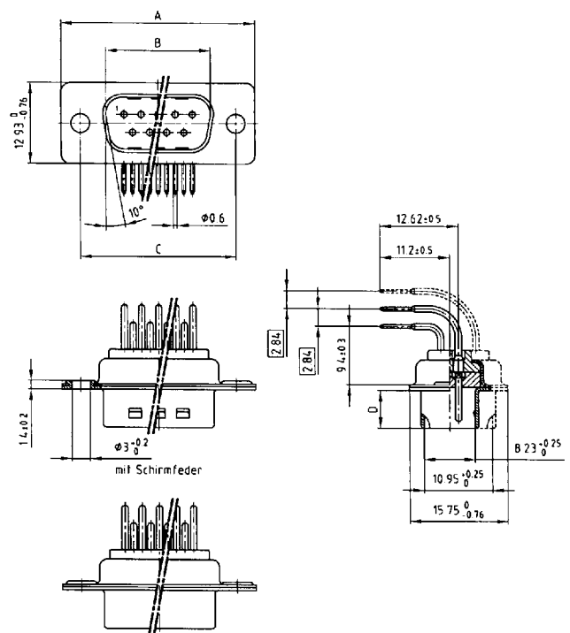
Plug connector
