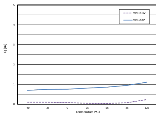
Figure 19. Off-state current vs. temperature
