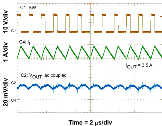
Figure 38. Output Ripple CCM
