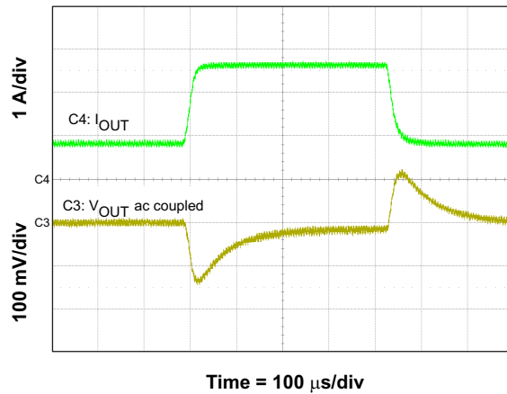
Figure 34. Load Transient
