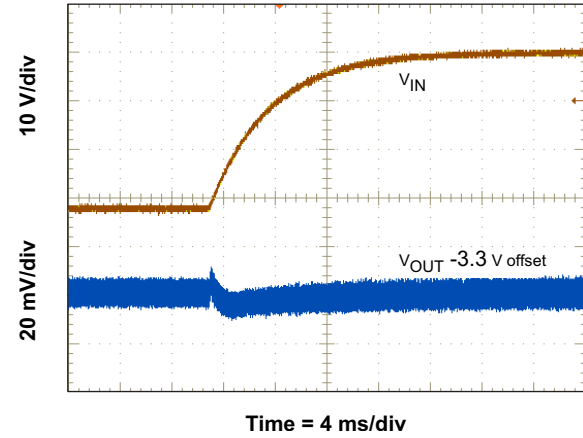
Figure 35. Line Transient (8 V to 40 V)
