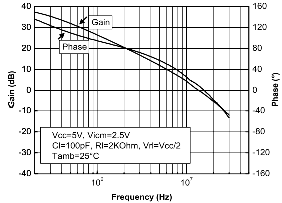
Figure 8. Voltage gain and phase vs. frequency at V_{CC} = 5 V and V_{icm} = 2.5 V
