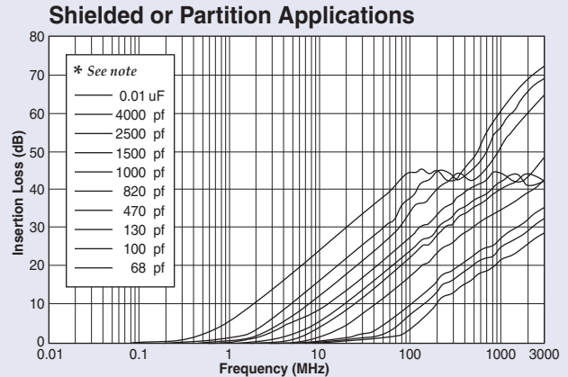
* Capacitance values for insertion loss curves are displayed left to right in the order shown.
