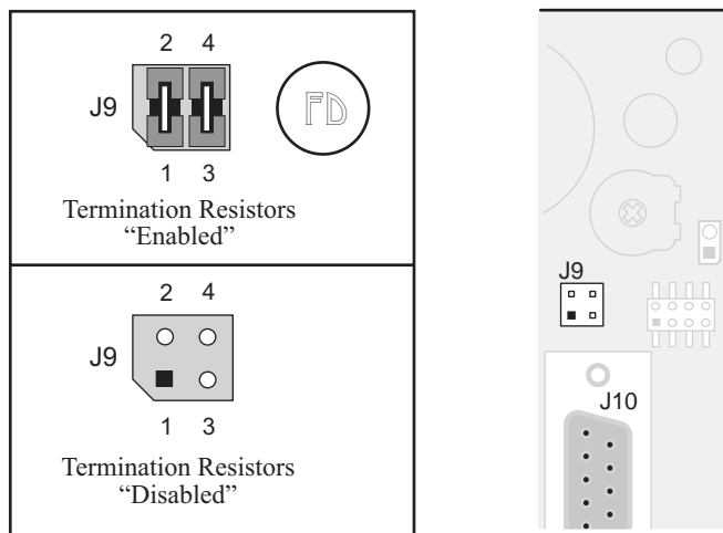
Figure 3-21. Enabling/Disabling Termination Resistors
