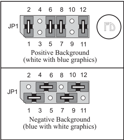
Figure 3-7. LCD Background Jumper Settings
