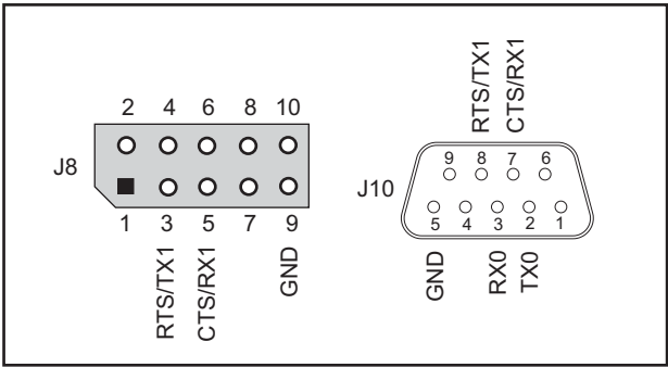
Figure 3-17. RS-232 Signals
