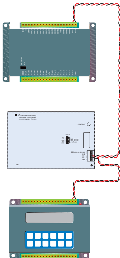
Figure 3-20. RS-485 Network
