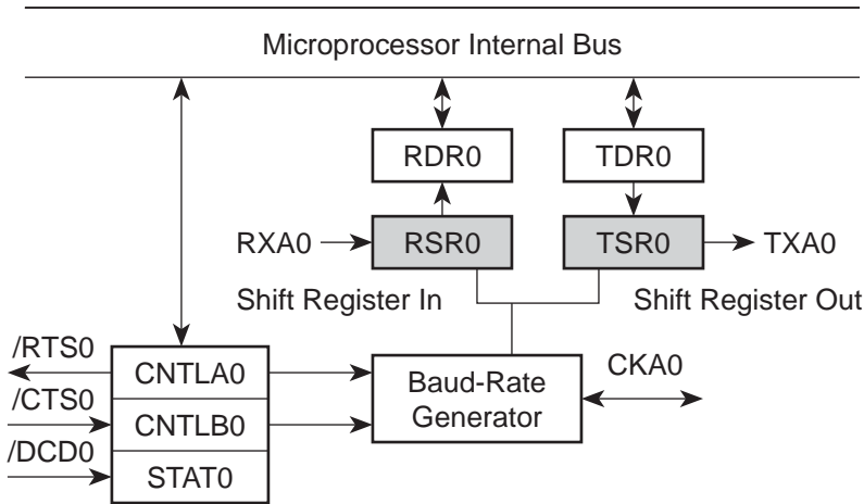
Figure 3-22. Z180 Serial Channel 0
