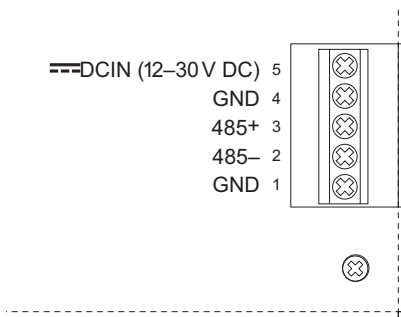
Figure 3-19. RS-485 Signals
