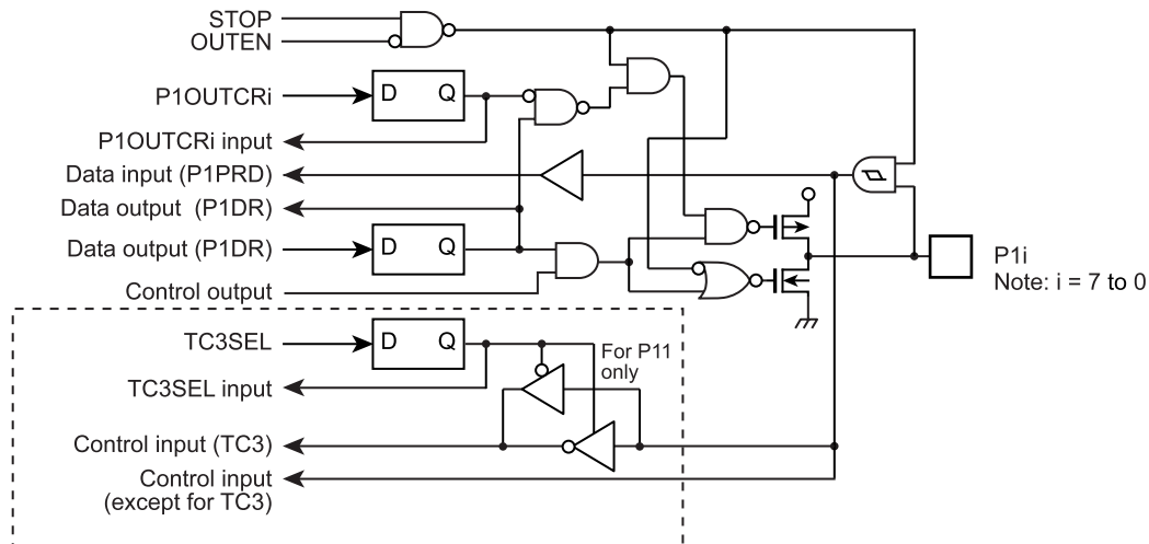
Figure 5-3 Port P1
