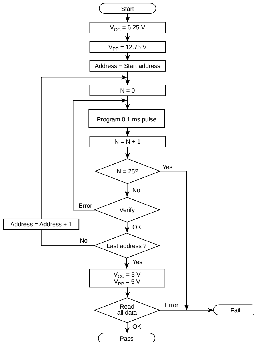
Figure 16-3 Programming Flowchart
