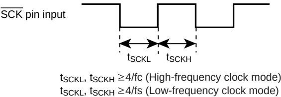
Figure 12-2 External Clock
