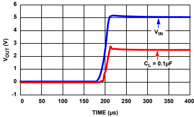
FIGURE 26. TURN-ON TIME WITH 0.1 \mu\text{F}
