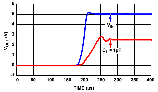
FIGURE 27. TURN-ON TIME WITH 1 \mu\text{F}
