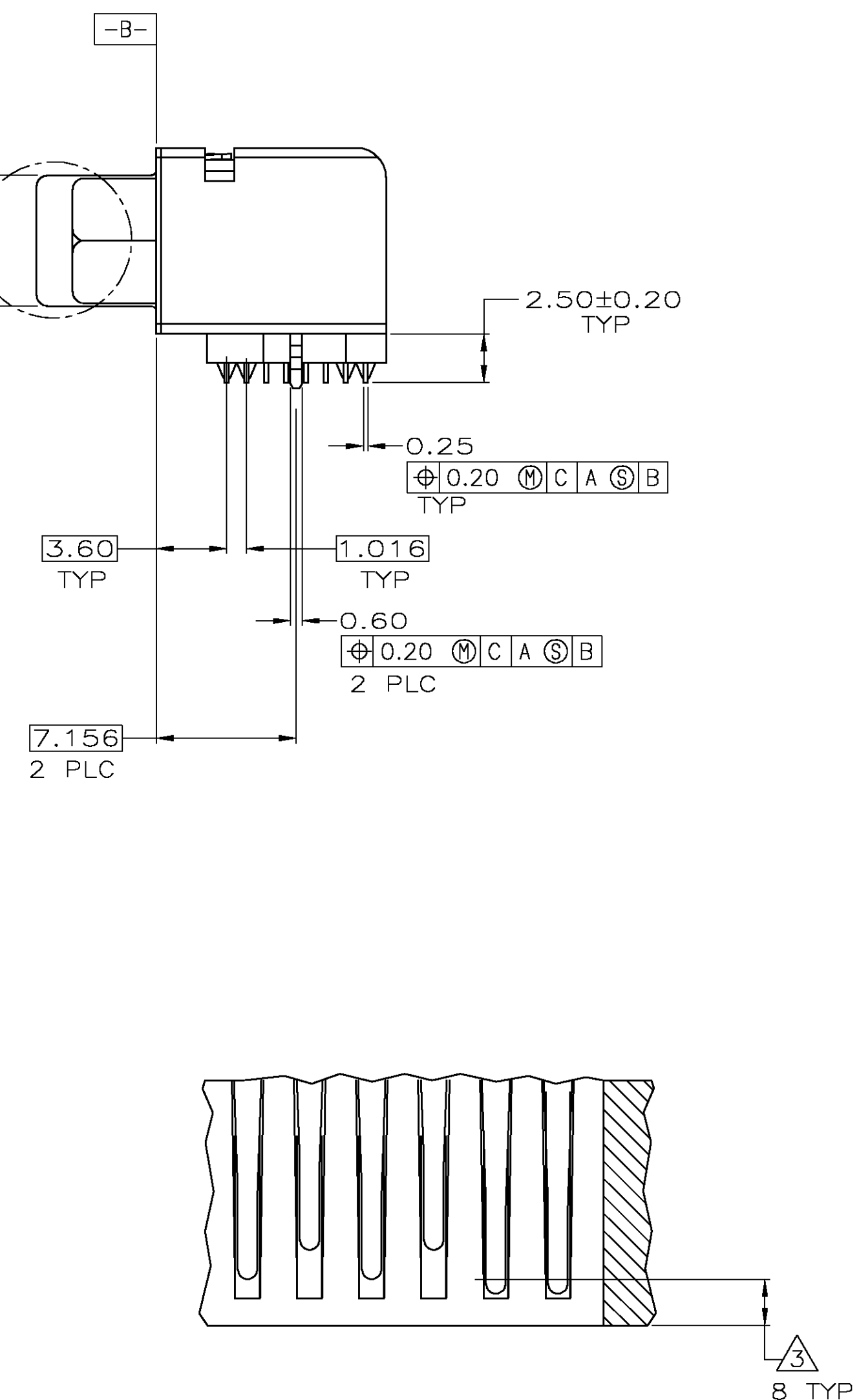
SECTION X-X SCALE 10:1
