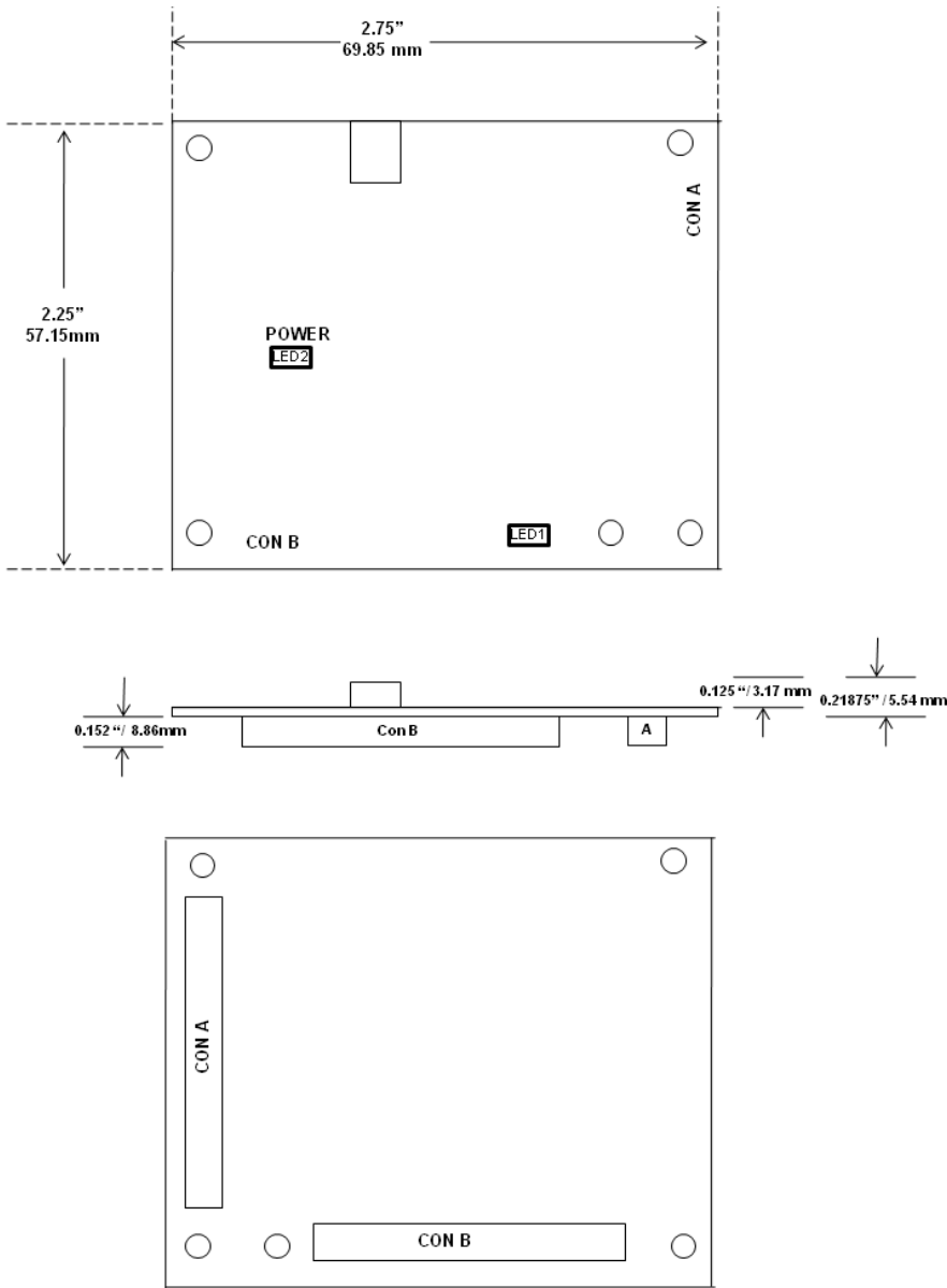
Figure 2-5. SDP Board Mechanical Specifications
