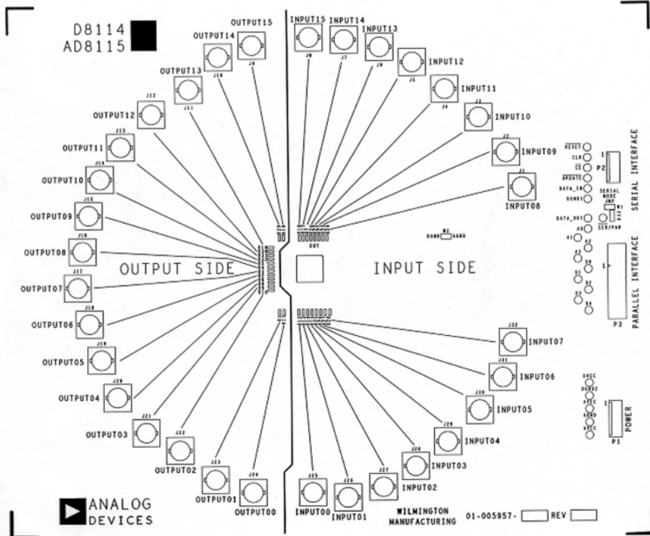
Figure 51. Component Side Silkscreen
