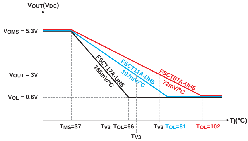
Fig. 3: Temperature slopes.
