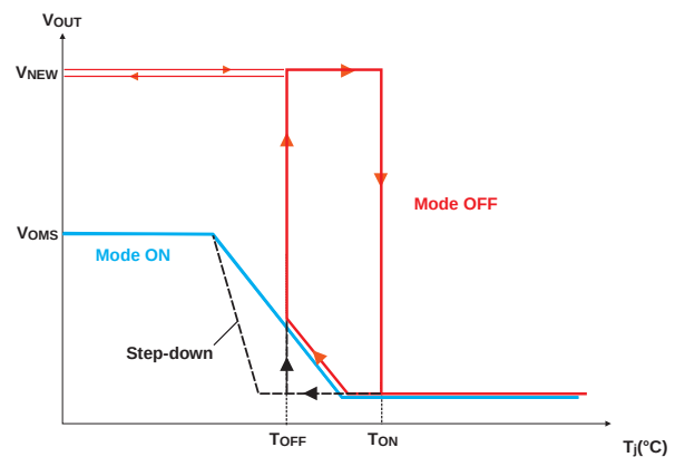
Fig. 12: Modified characteristics.
