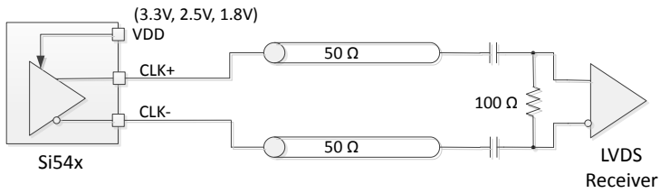
AC-Coupled LVDS
