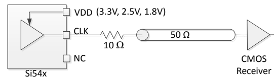
Single CMOS Termination
