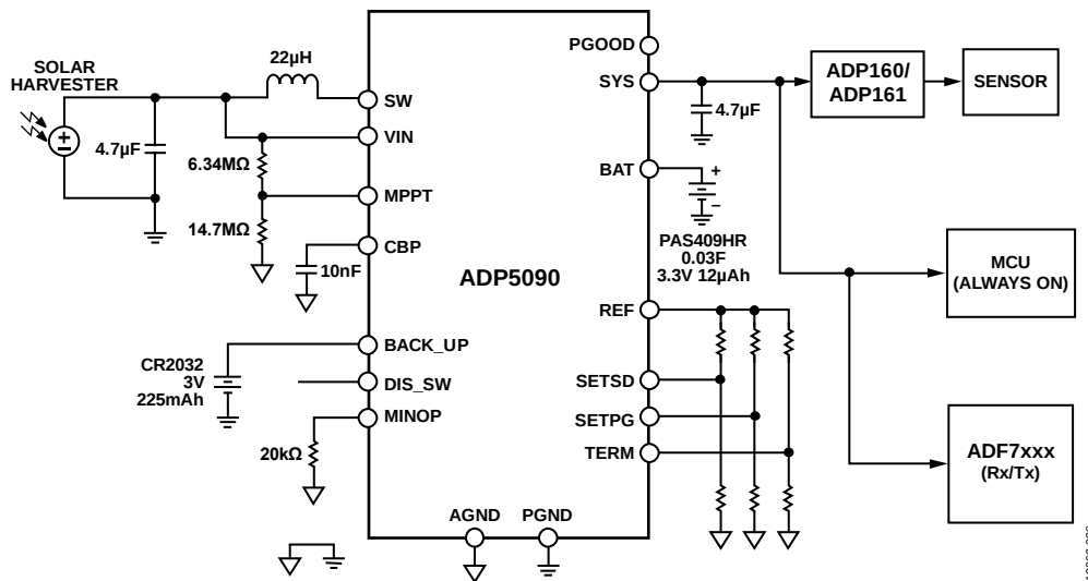
Figure 33. ADP5090 Based Energy Harvester Wireless Sensor Application with PV Cell as the Harvesting Energy Source (Trony 0.7 V, 60 \mu A, Alta Devices 0.72 V, 42 \mu A, Gcell 1.1 V, 100 \mu A), Shoel Electronics Polyacene Coin Type Capacitor PAS409HR as the Harvested Energy Storage, and Panasonic Primary Li-Ion Coin Cell CR2032 as the Backup Battery
